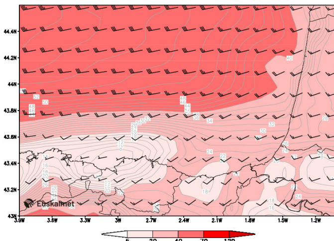
Haizea azalean (km/h) 2026/01/09 12:00 Viento superficial (km/h)
