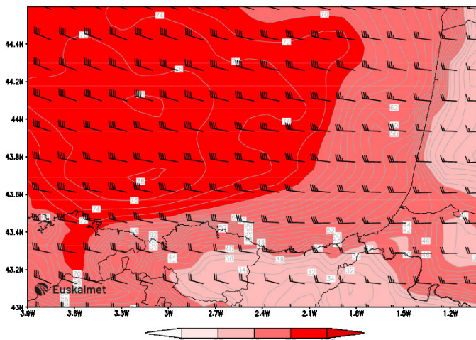
Haizea azalean (km/h) 2026/01/10 12:00 Viento superficial (km/h)
